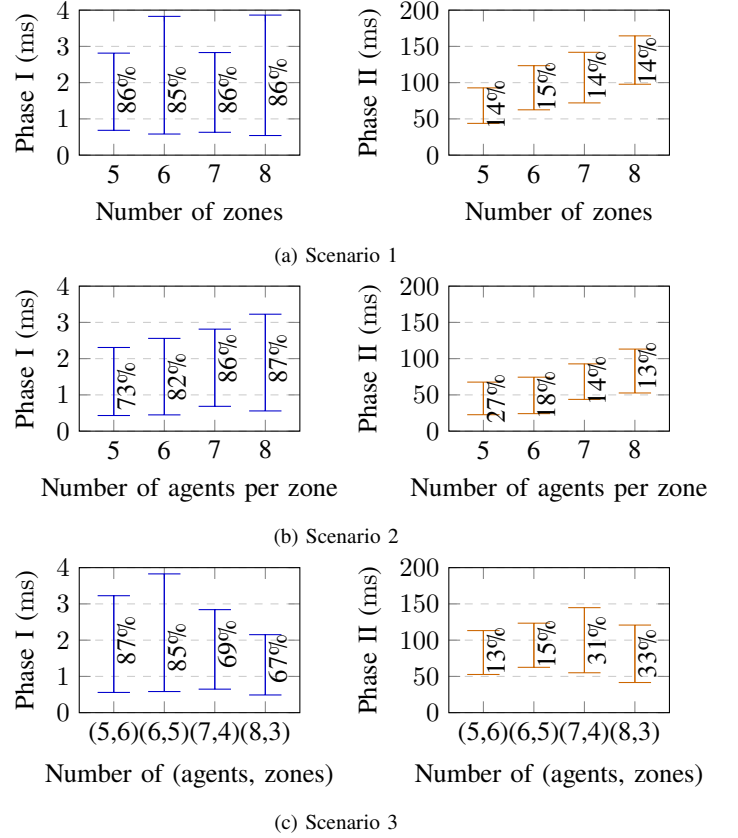
Fig. 4. The local end-to-end latency L for Phase I, the global end-to-end latency E for Phase II and failure ratio F as percentage for different values of ECUs per zone (agents) A and number of zones Z . (a) Scenario 1: A = 5 and Z varies; (b) Scenario 2: Z = 5 and A varies; and (c) Scenario 3: A and Z varies inversely. The failure ratio F decreases when the number of agents per zone A increases.
