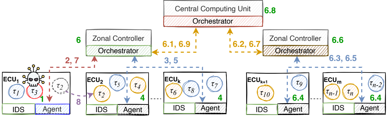
Fig. 2. Workflow of SHIFTGUARD that starts with an attack detection of \tau_3 (Step 1) and ends with migration of \tau_2 in ECU_2 (Step 8). SHIFTGUARD operates in two phases: (a) first it checks if migration is feasible in the local zone (Phase I) and (b) if not, finds an ECU in another zone, which involves orchestrators in other zonal controllers and central computing unit (Phase II).
