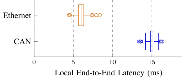
Fig. 11. Comparison of end-to-end migration latency L using CAN and Ethernet. Ethernet achieves approximately 50% lower latency compared to CAN due to higher bitrate.
